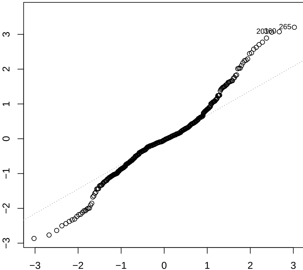
Q-Q Residuals
