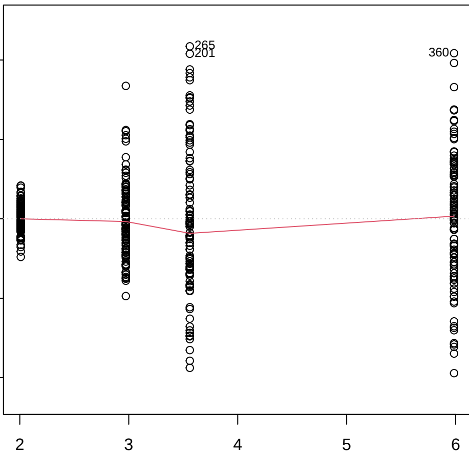
Residuals vs Fitted
