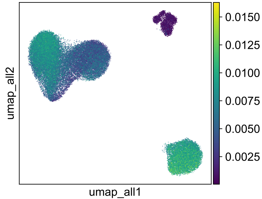
activation_all
