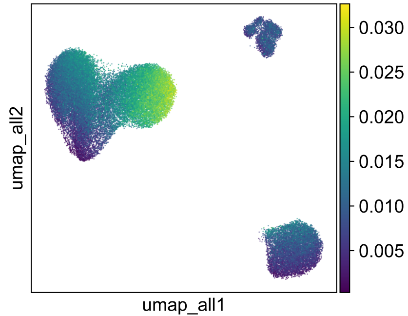
exhaustion_all
