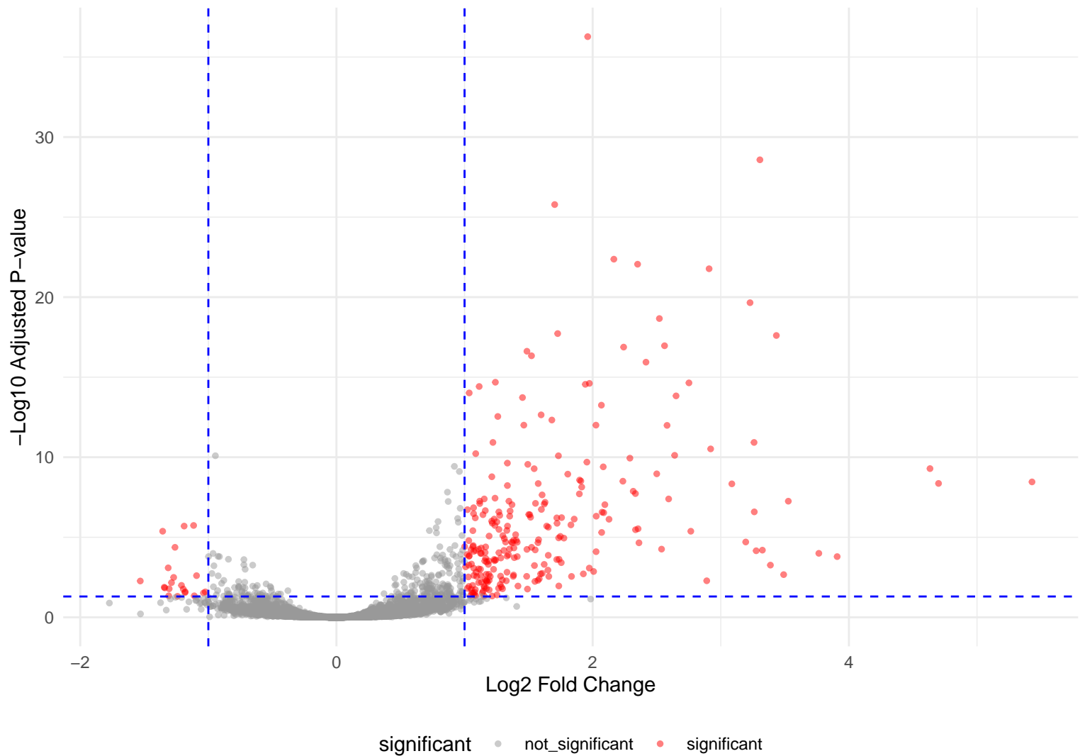
Volcano Plot – treatment
