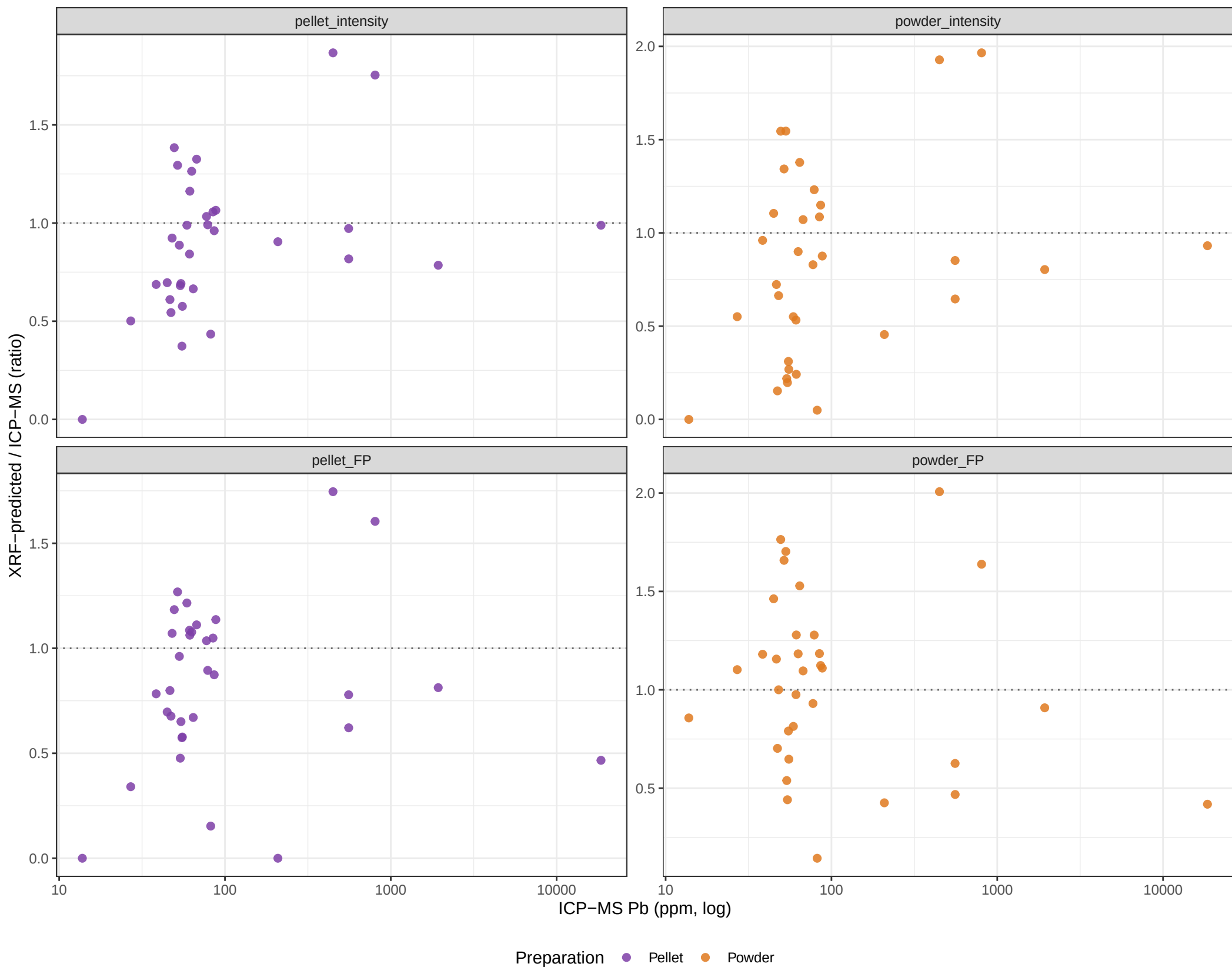
Method agreement: XRF/ICP-MS ratio vs ICP-MS reference
