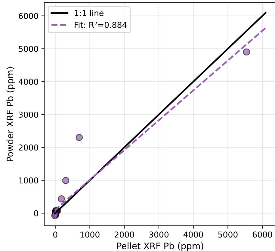
C. Powder vs Pellet ( r=0.940 , n=24 )
