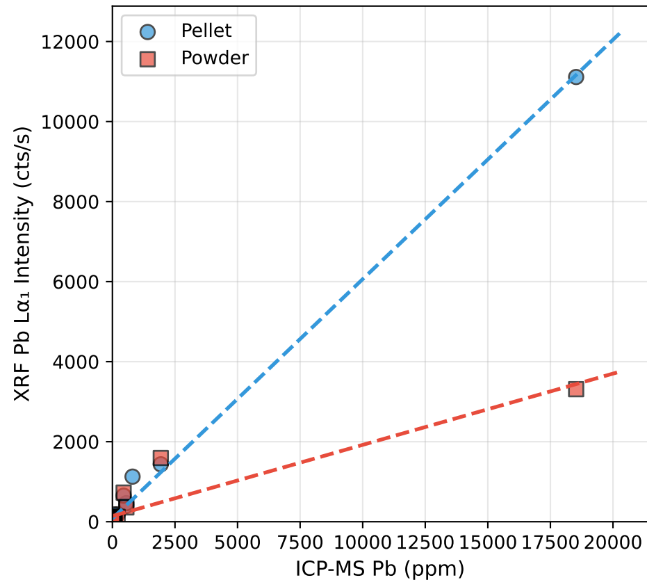
A. Raw XRF Intensity vs ICP-MS
