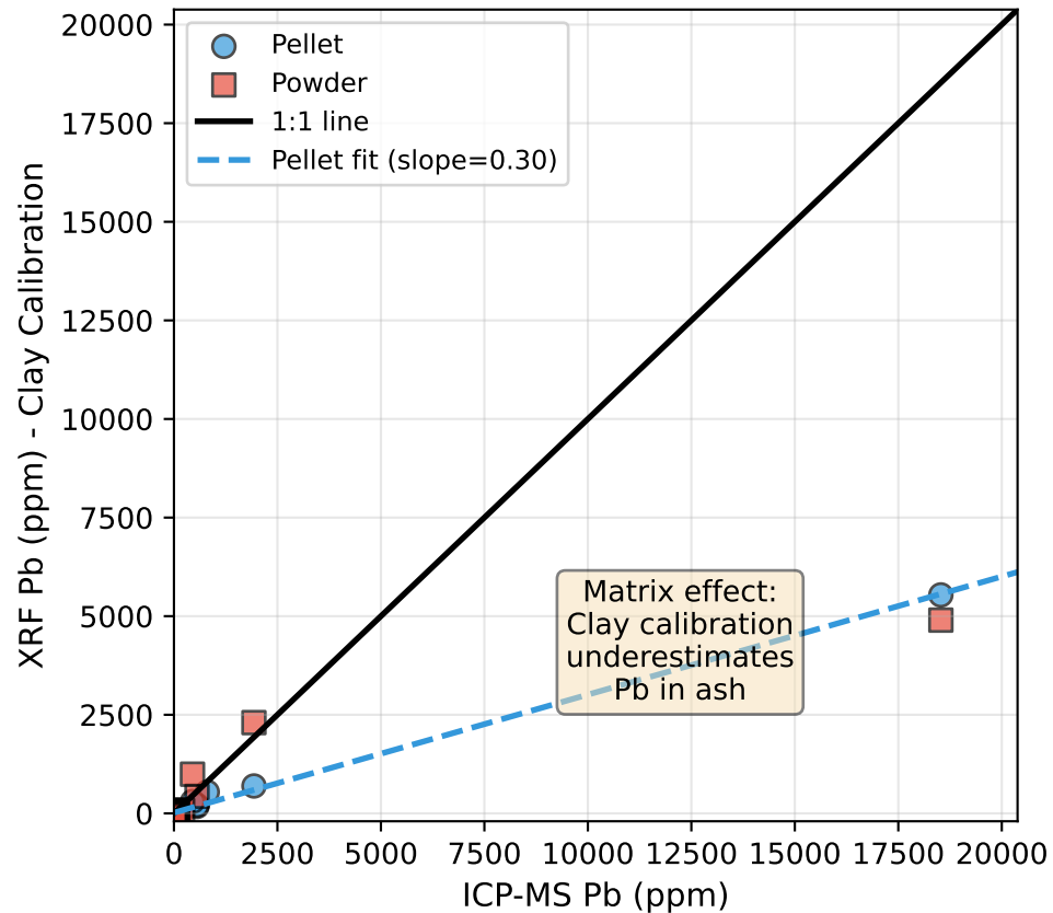
B. Clay-Calibrated XRF vs ICP-MS (Shows Matrix Effect)
