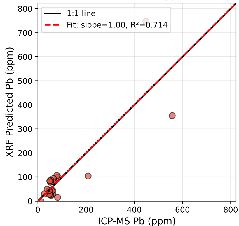
POWDER - Validation CV-RMSE = 177 ppm
