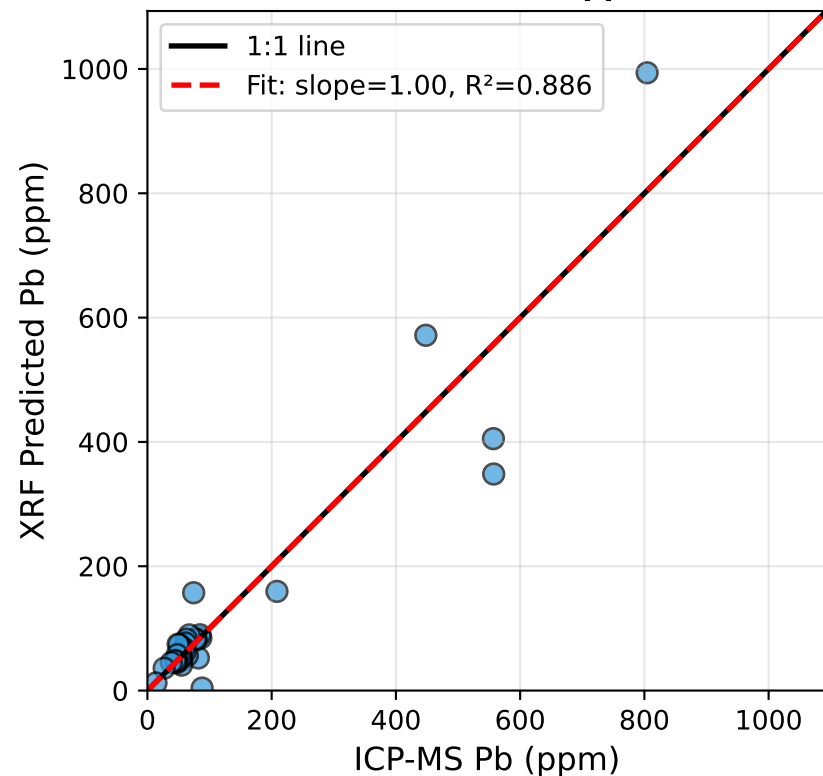
PELLET - Validation CV-RMSE = 101 ppm
