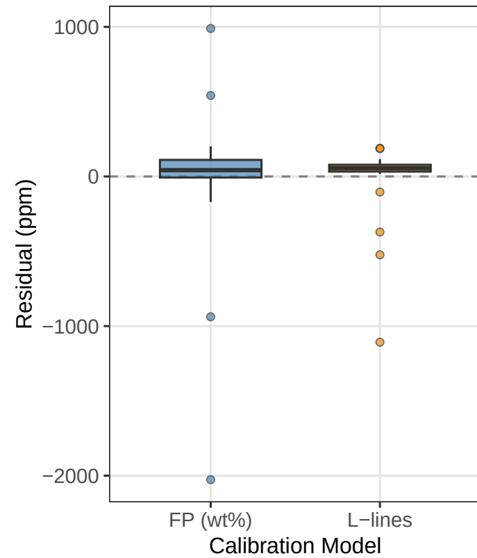
Model Residuals
