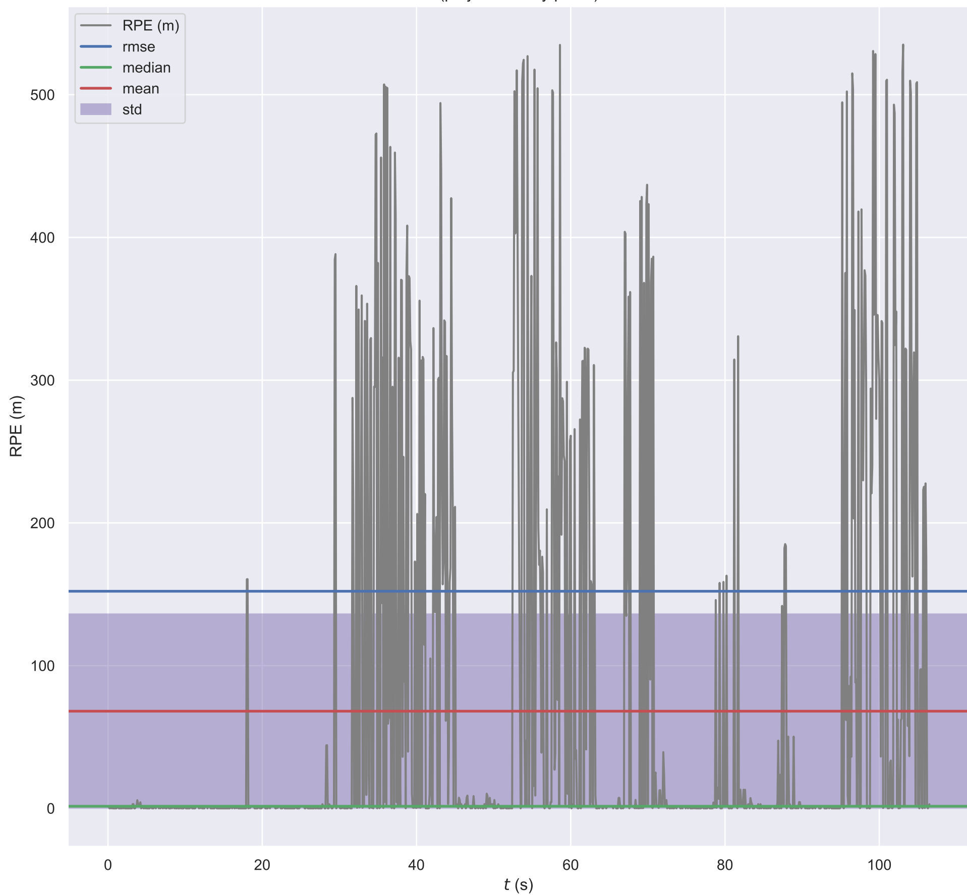
RPE w.r.t. translation part (m) for \delta = 1 (frames) using consecutive pairs (not aligned) (projected to xy plane)
