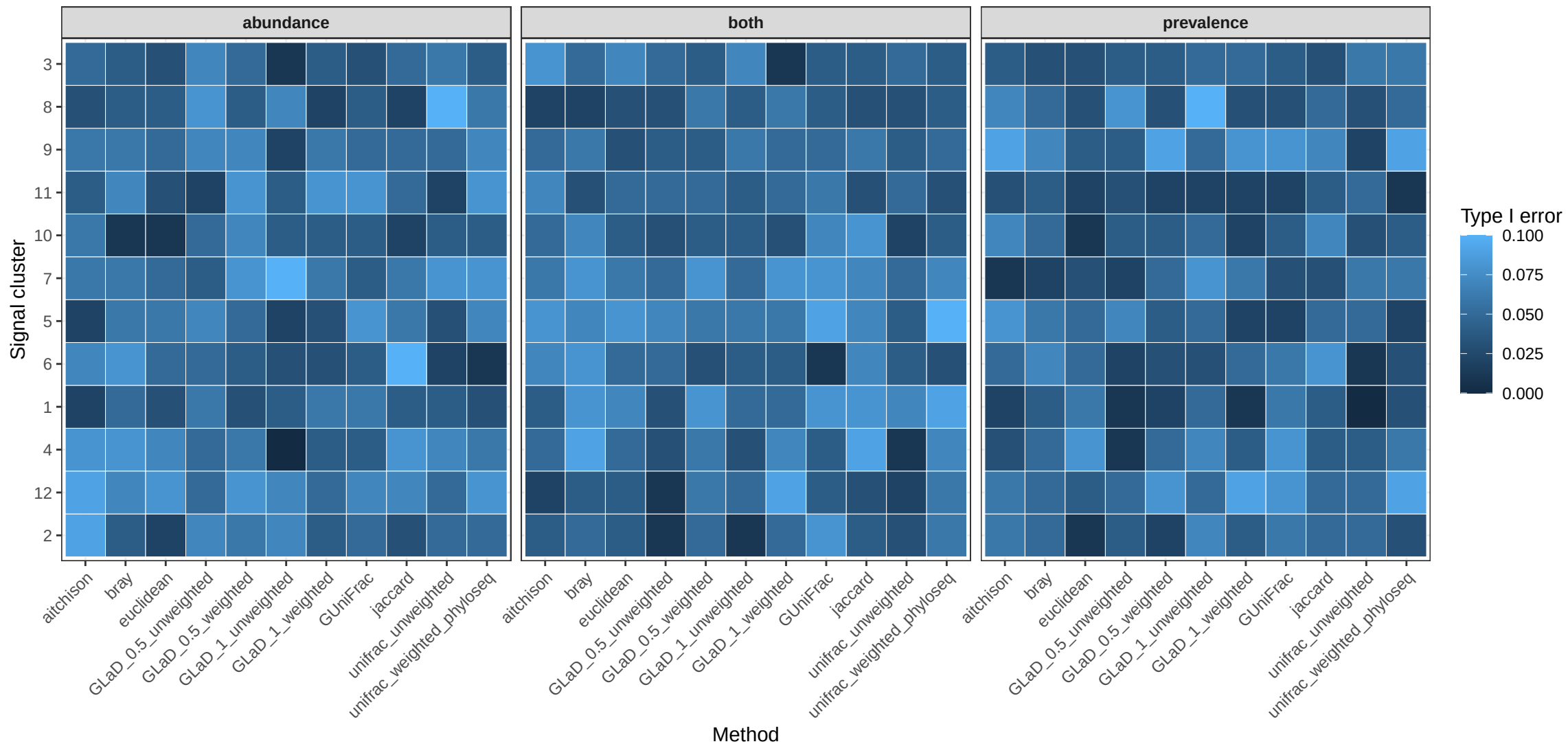
Type I error heatmap | k = 12 | \beta = 0
