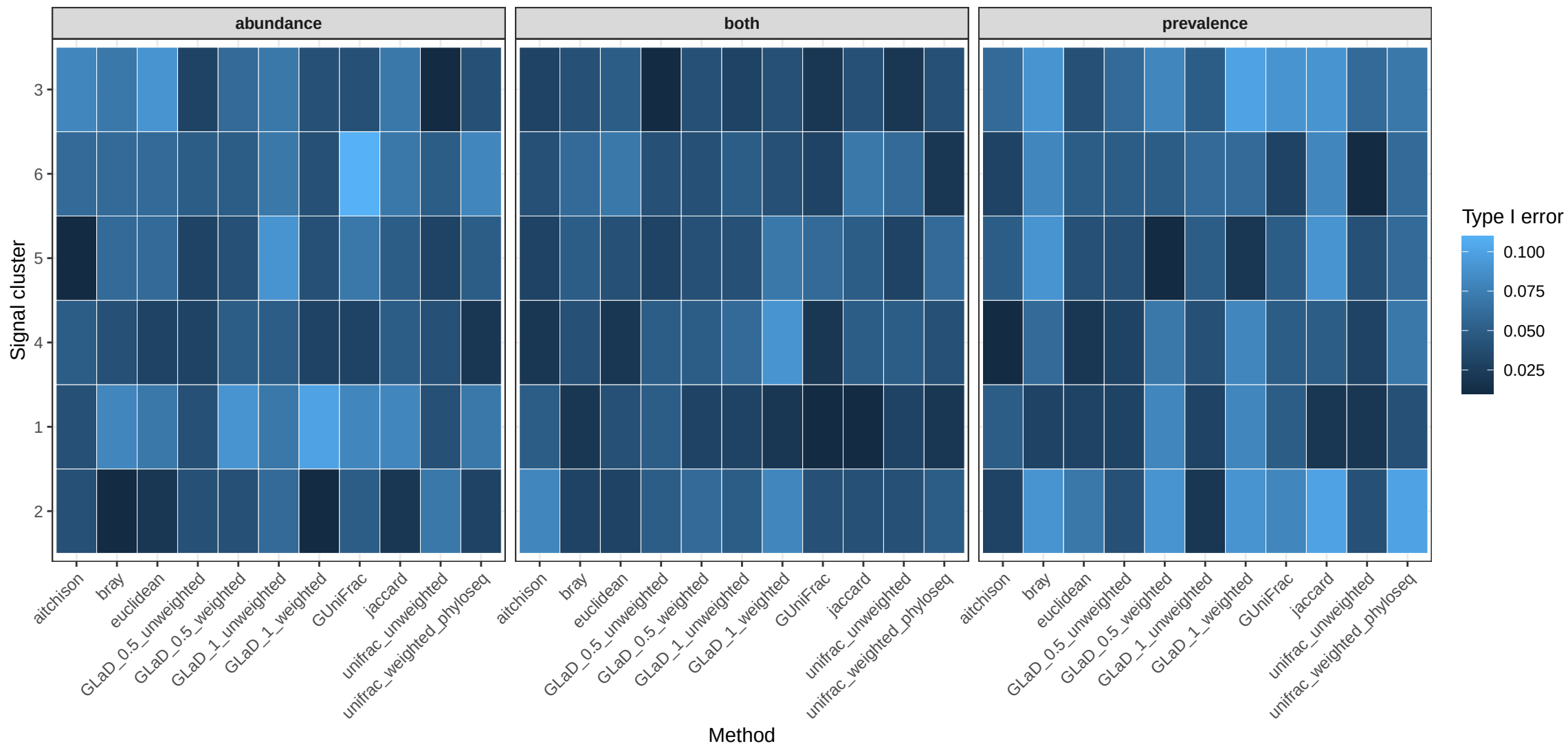
Type I error heatmap | k = 6 | beta = 0
