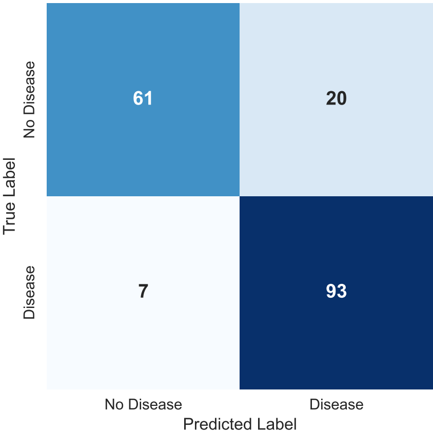
Confusion Matrix
