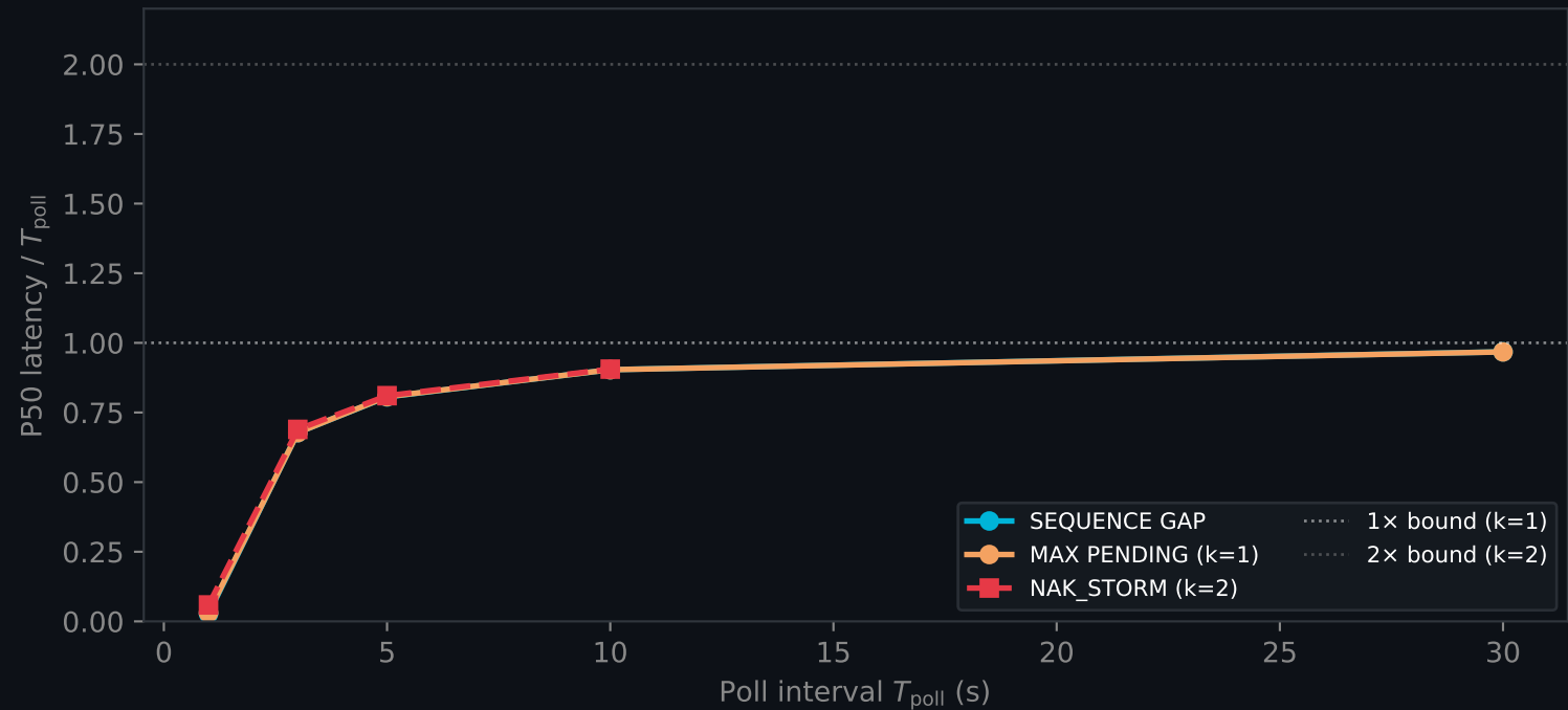
Theorem 2 Validation: Latency \leq k \times T_{\text{poll}} for k \in \{1, 2\}
