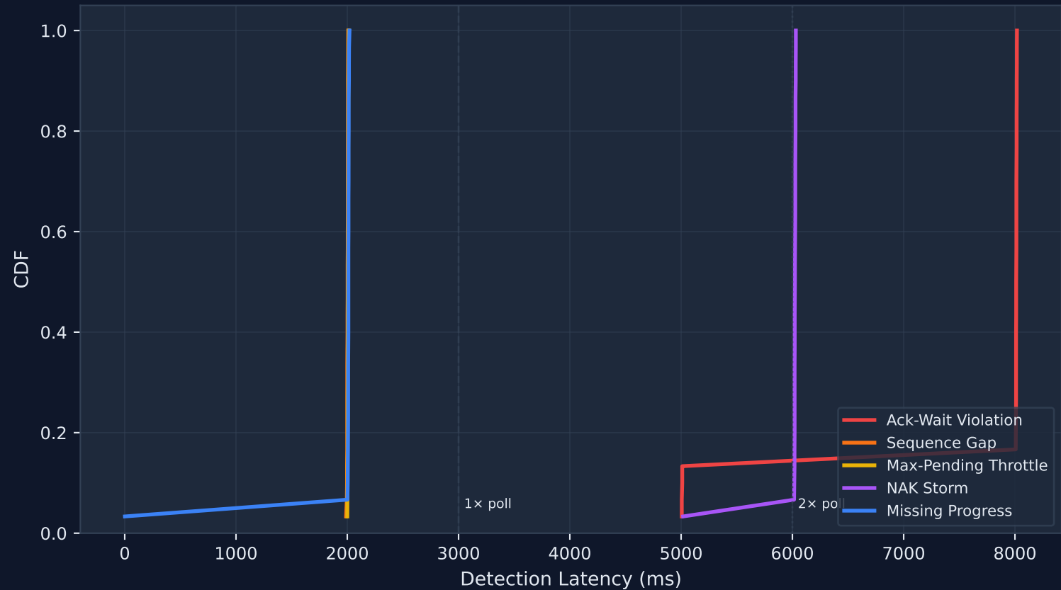
Figure 2: Detection Latency CDF by Violation Type (time from violation injection to first nats-lens event)
