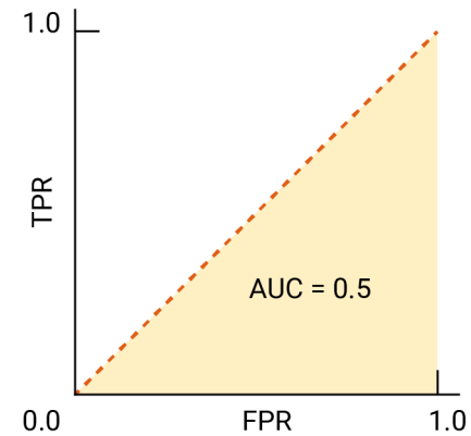
ROC and AUC of completely random guesses
