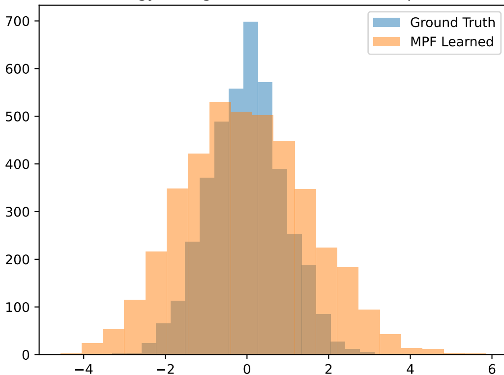
Energy Histogram for Entire Partition Space
