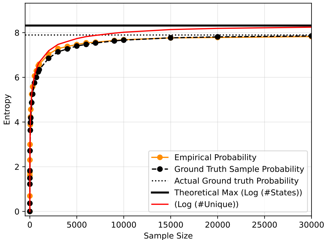
Entropy vs Sample Size: Problem=[6 Positions, 4 Letters]
