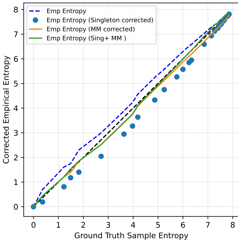
Entropy Correction: Problem=[6 Positions, 4 Letters]
