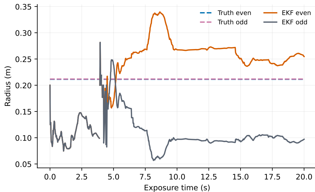
C Reconstructed radii
