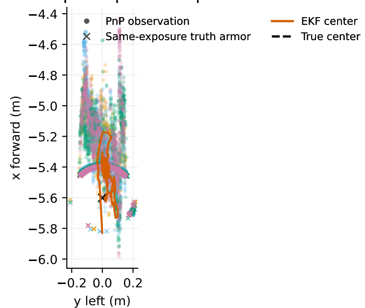
D Top view (x-forward points upward; color = armor slot) 360 slot switches | median |radial| 0.207 m | transverse 0.007 m
