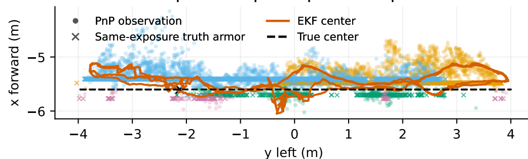
D Top view (x-forward points upward; color = armor slot) 539 slot switches | median |radial| 0.145 m | transverse 0.008 m
