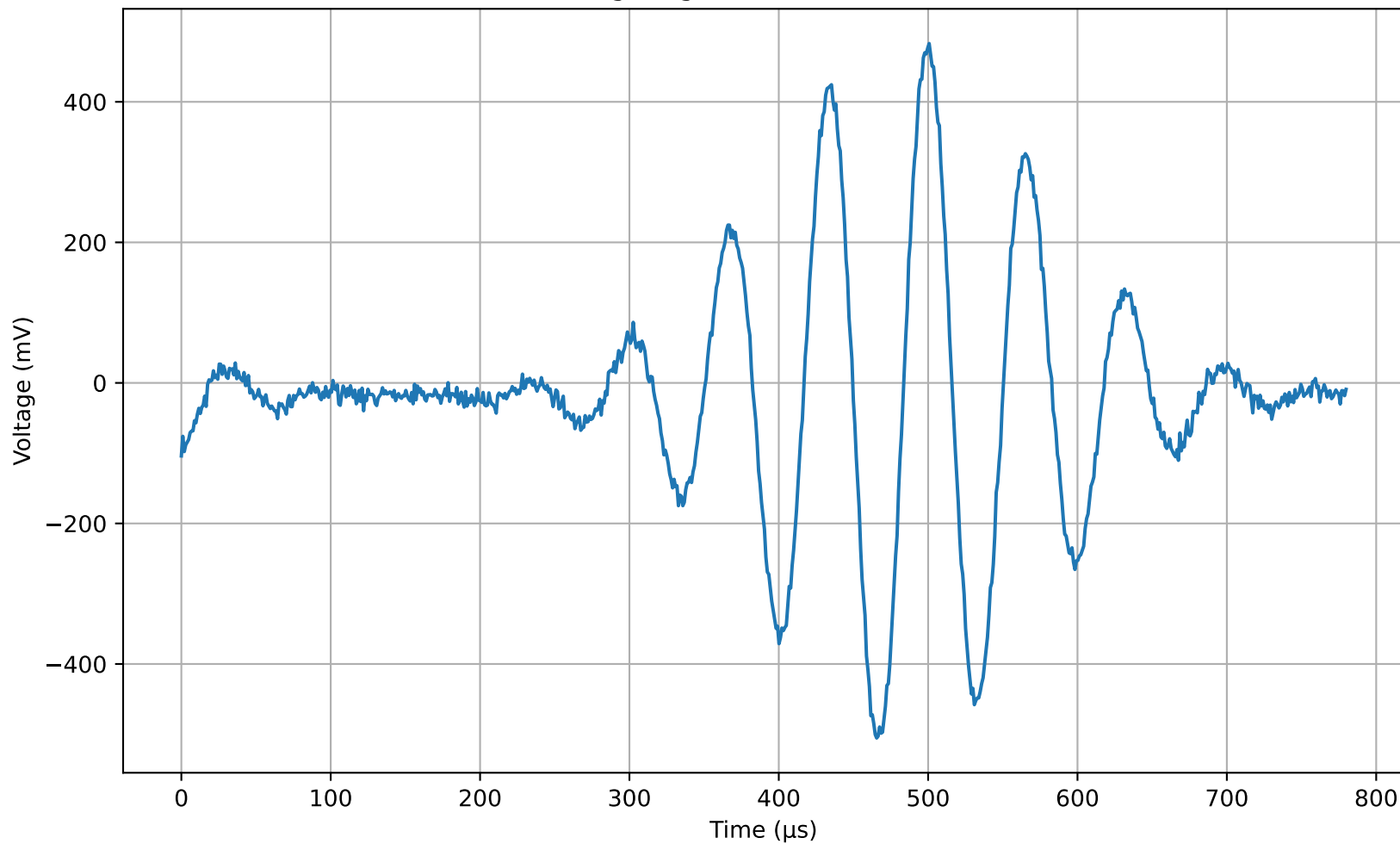
PICO signal generation - 15000.0 Hz
