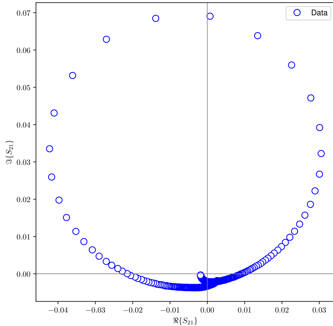
I-Q Plot
