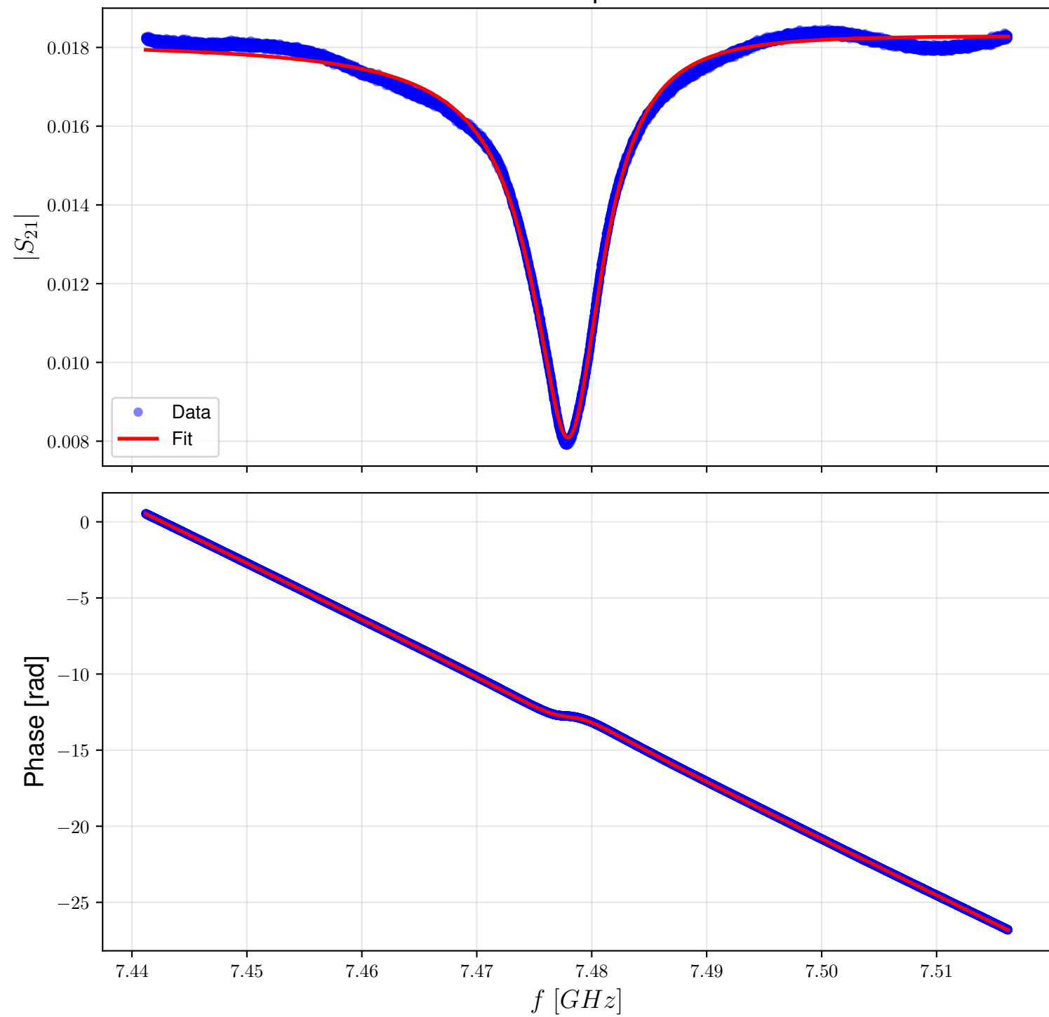
Resonance Fit - Temperature: 1000mK
