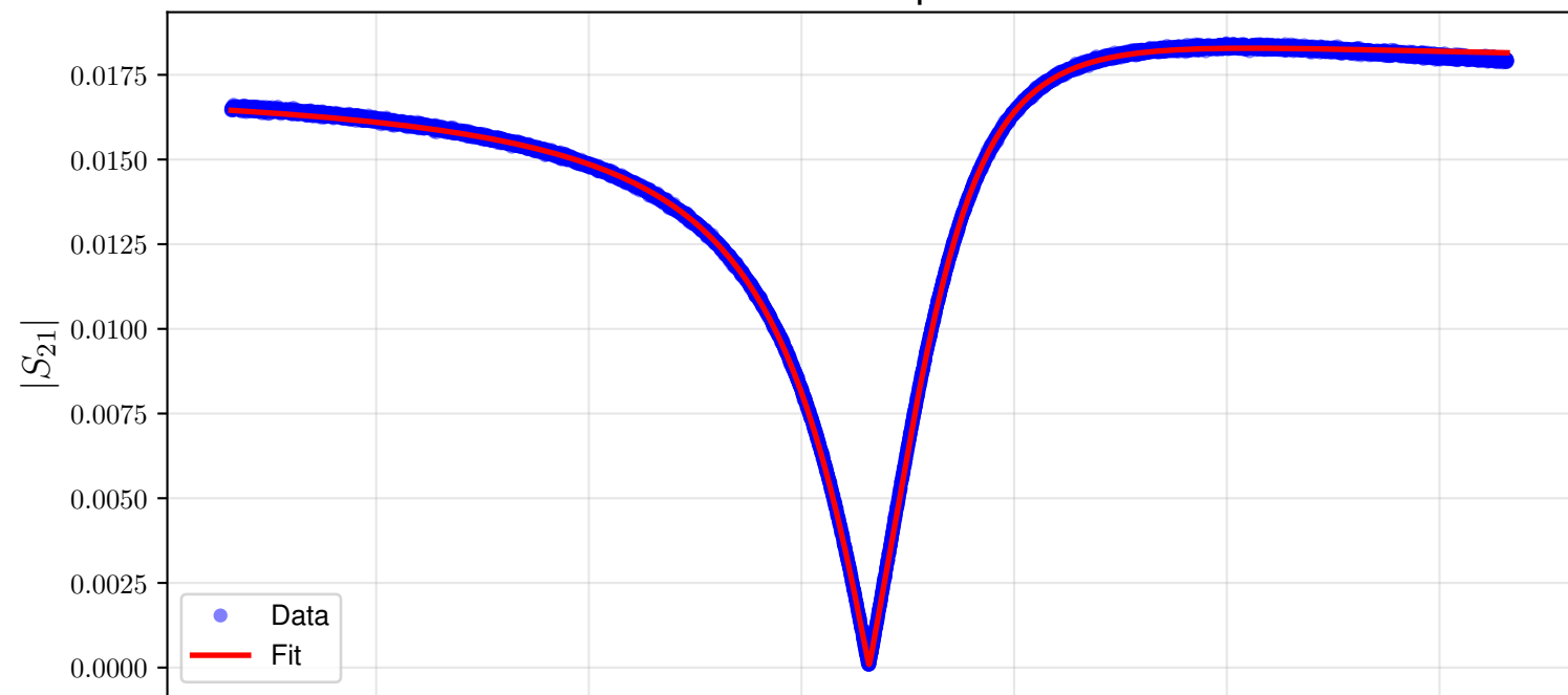
Resonance Fit - Temperature: 10mK
