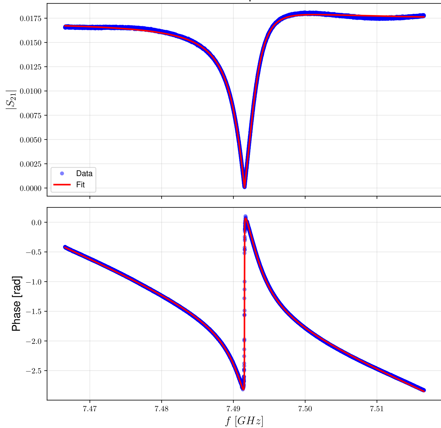
Resonance Fit - Temperature: 300mK_b
