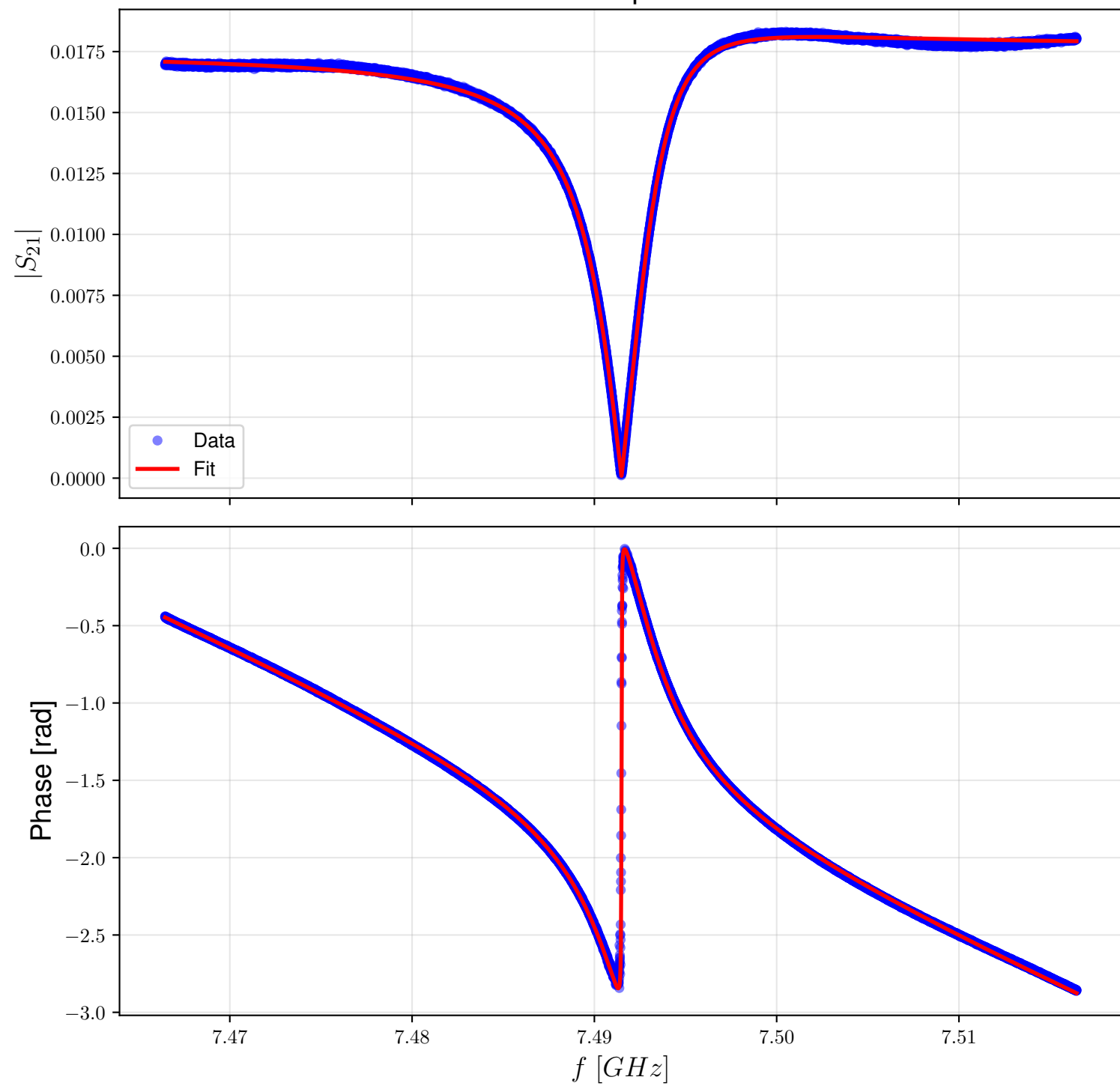
Resonance Fit - Temperature: 500mK_b
