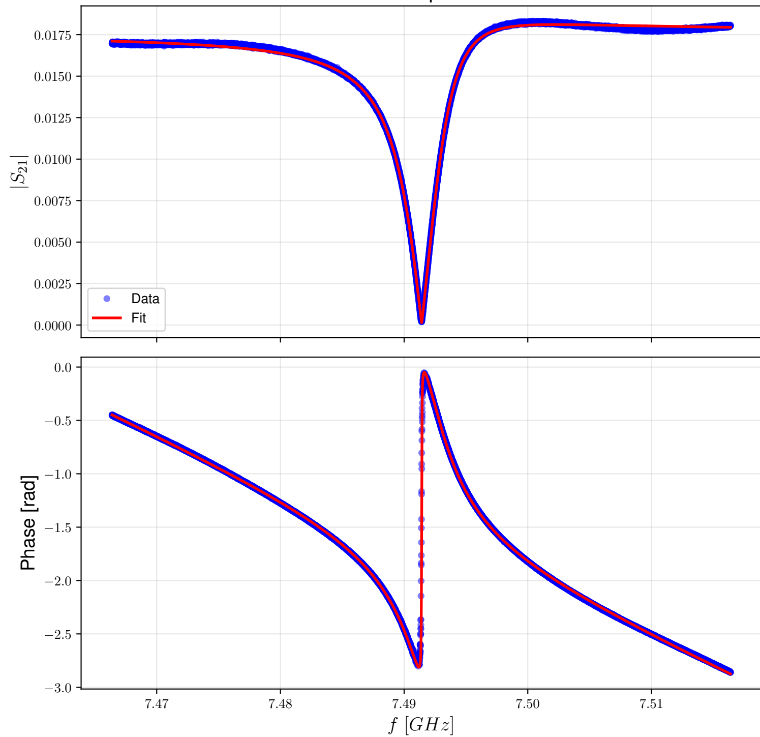
Resonance Fit - Temperature: 550mK_b
