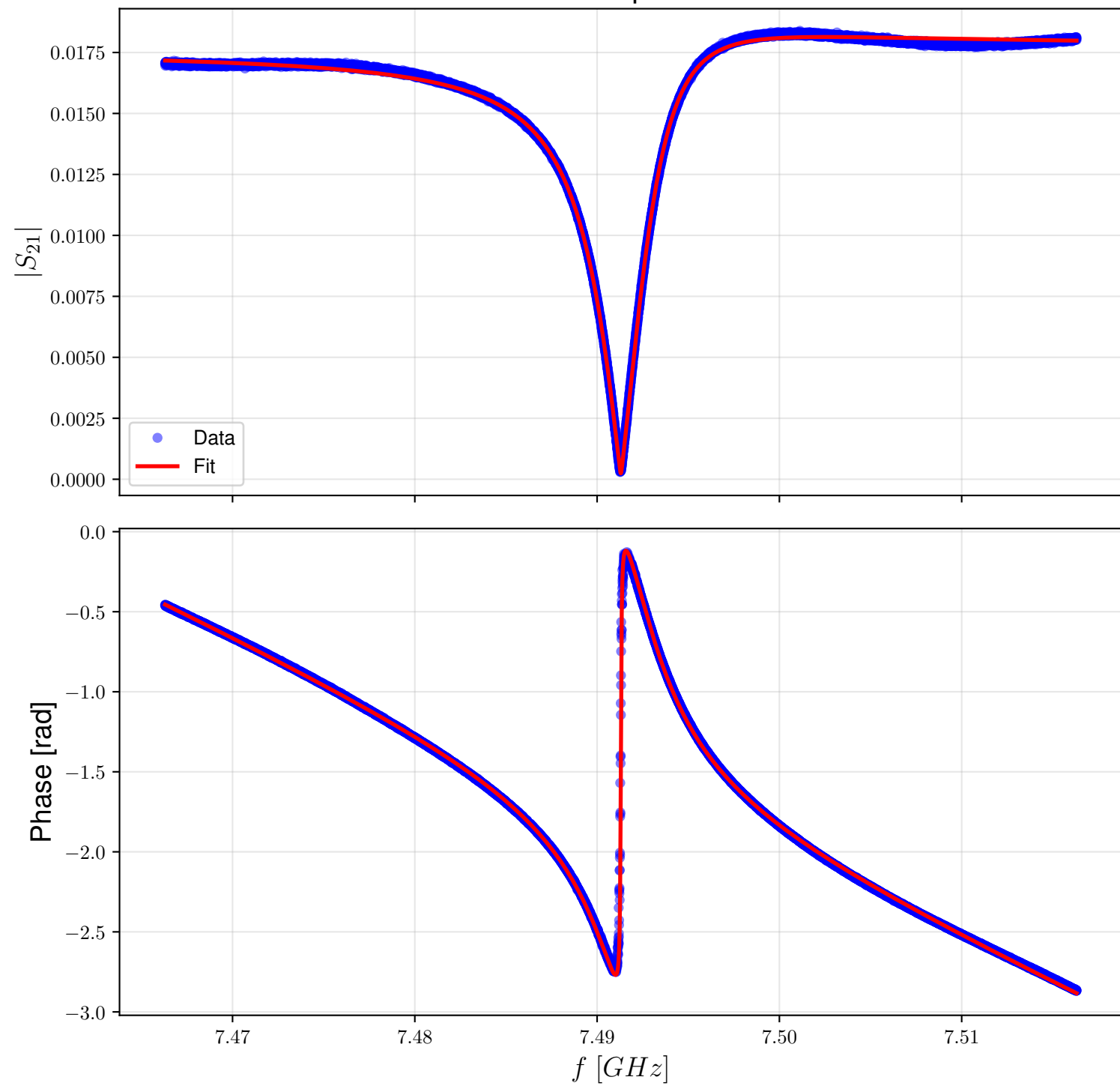
Resonance Fit - Temperature: 600mK_b
