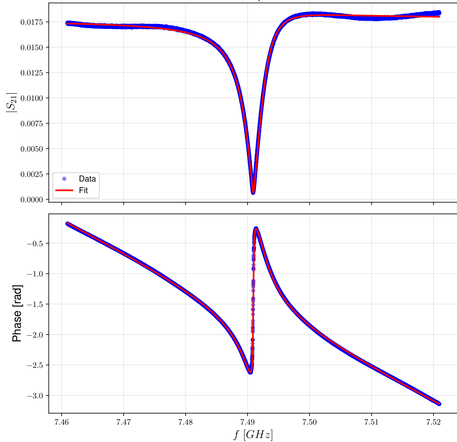
Resonance Fit - Temperature: 650mK_b
