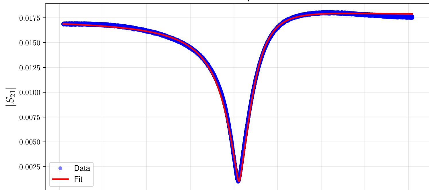
Resonance Fit - Temperature: 700mK
