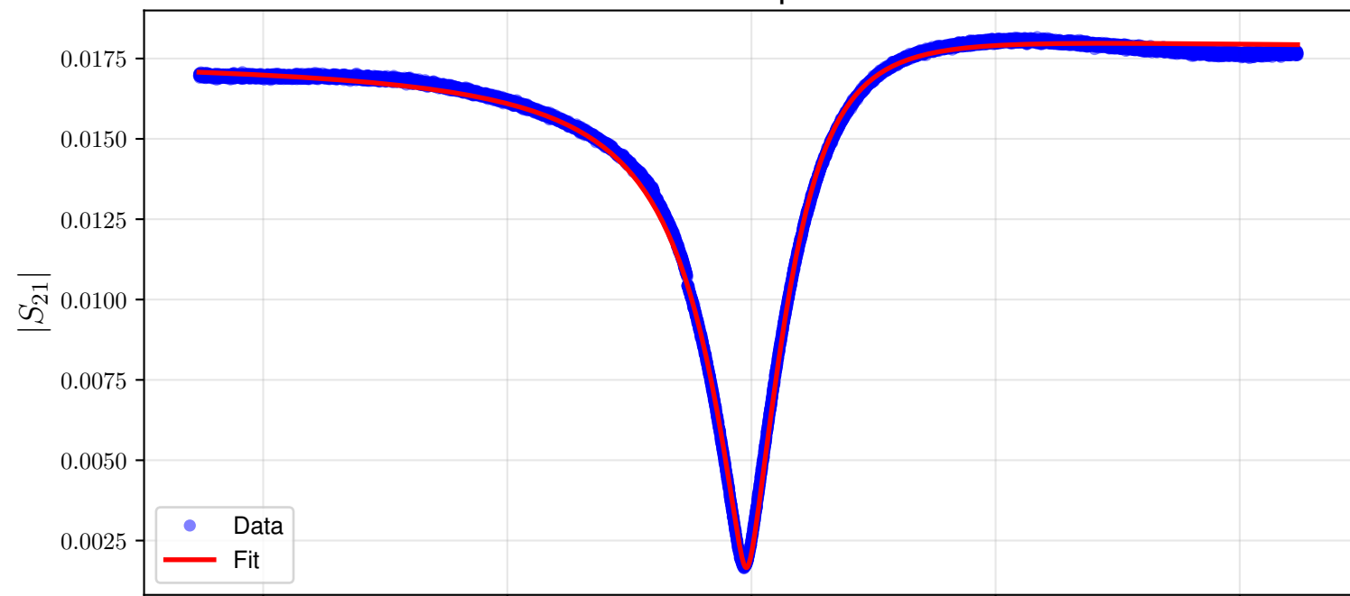
Resonance Fit - Temperature: 750mK
