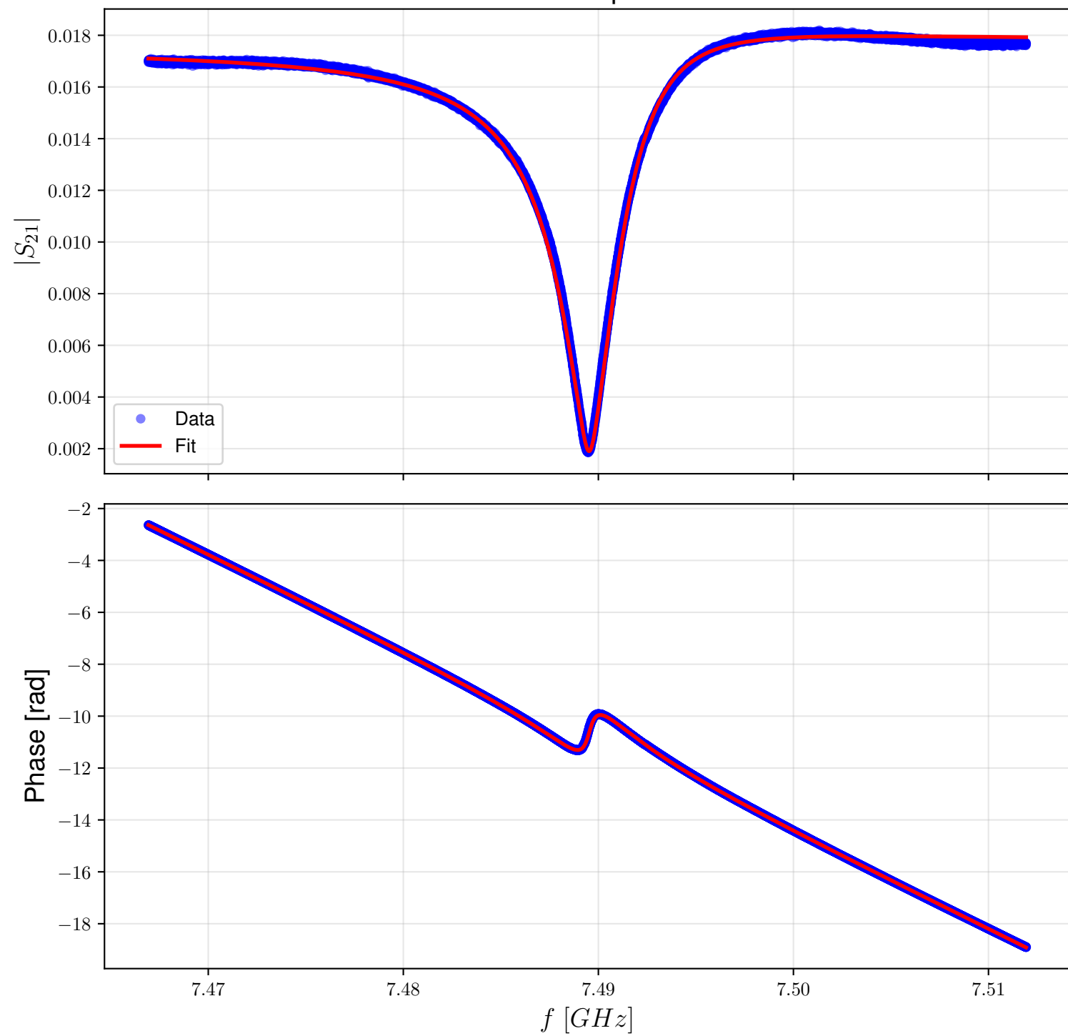
Resonance Fit - Temperature: 775mK
