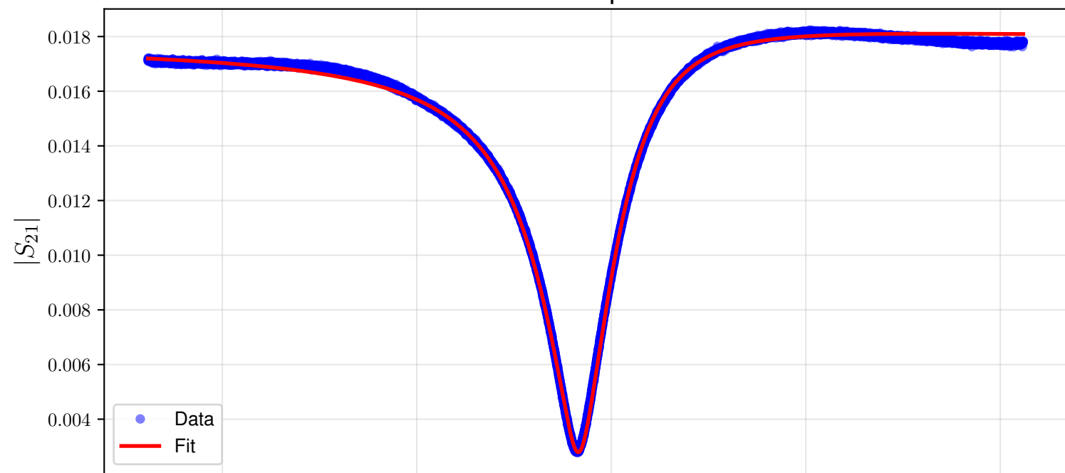
Resonance Fit - Temperature: 825mK
