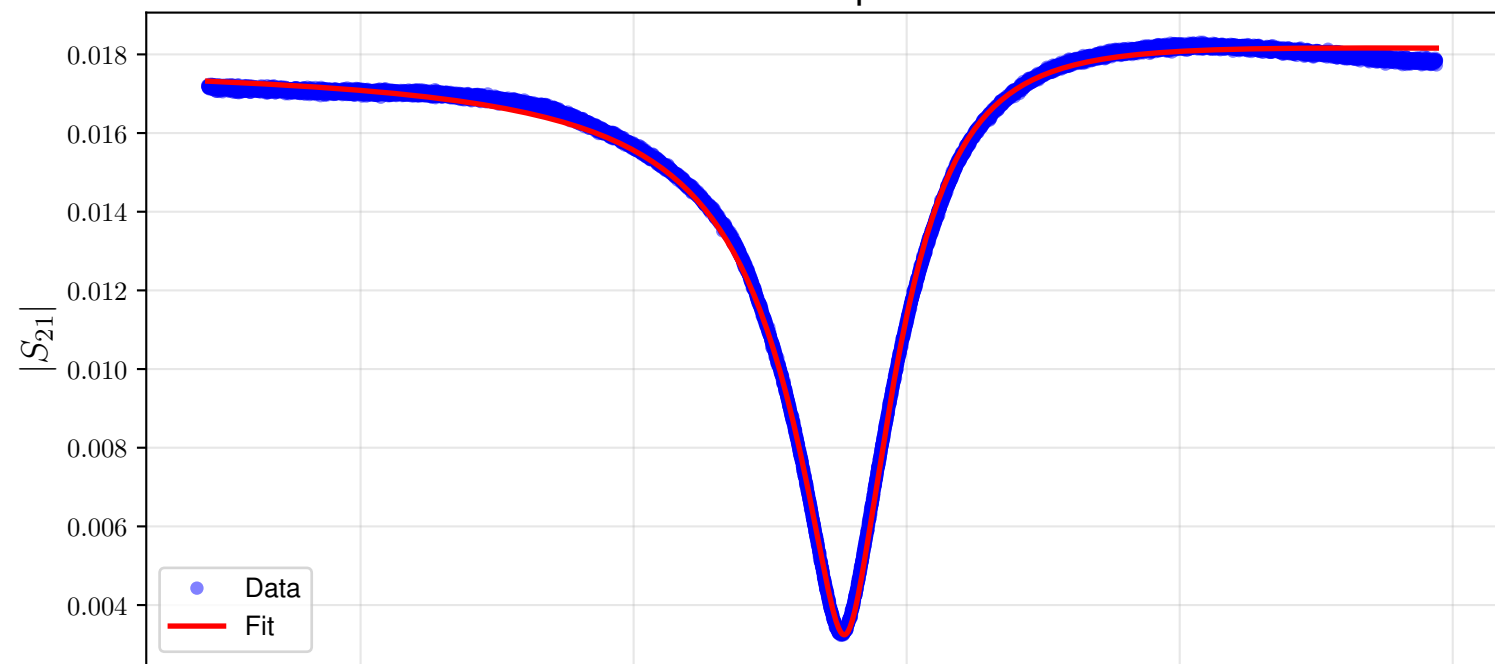
Resonance Fit - Temperature: 850mK
