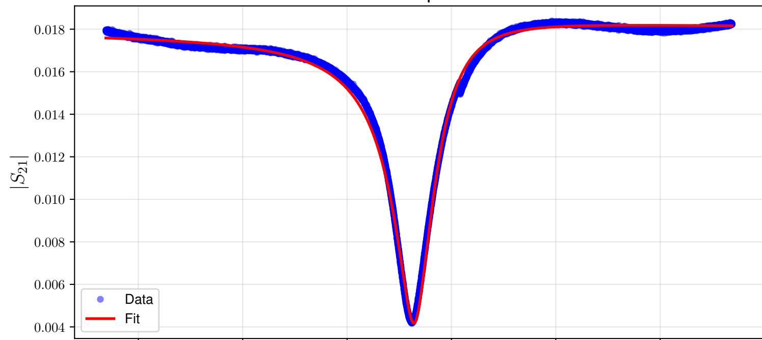
Resonance Fit - Temperature: 875mK_b
