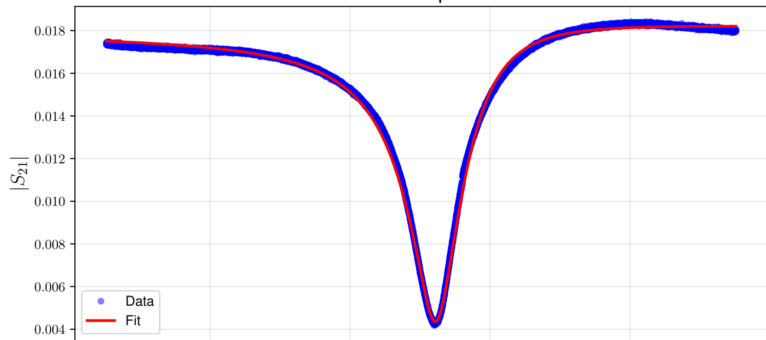
Resonance Fit - Temperature: 900mK
