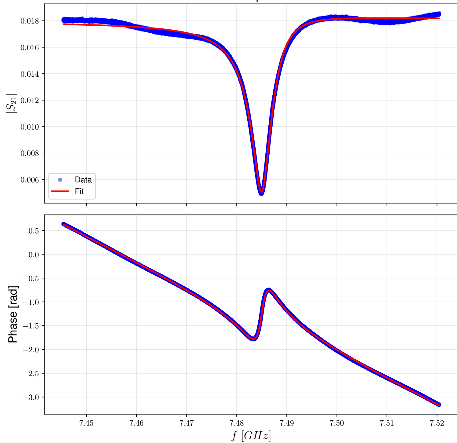
Resonance Fit - Temperature: 925mK_b
