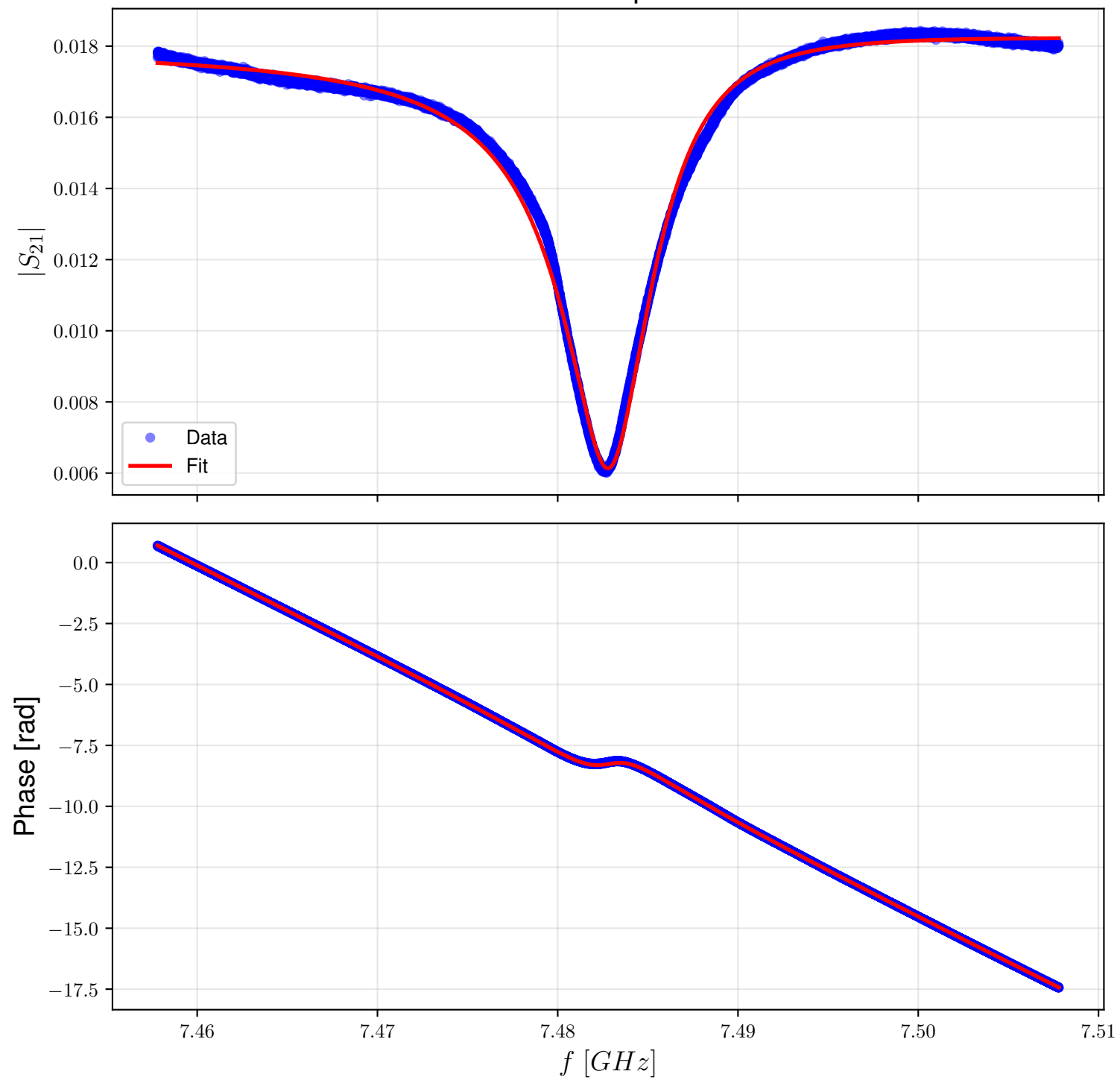
Resonance Fit - Temperature: 950mK
