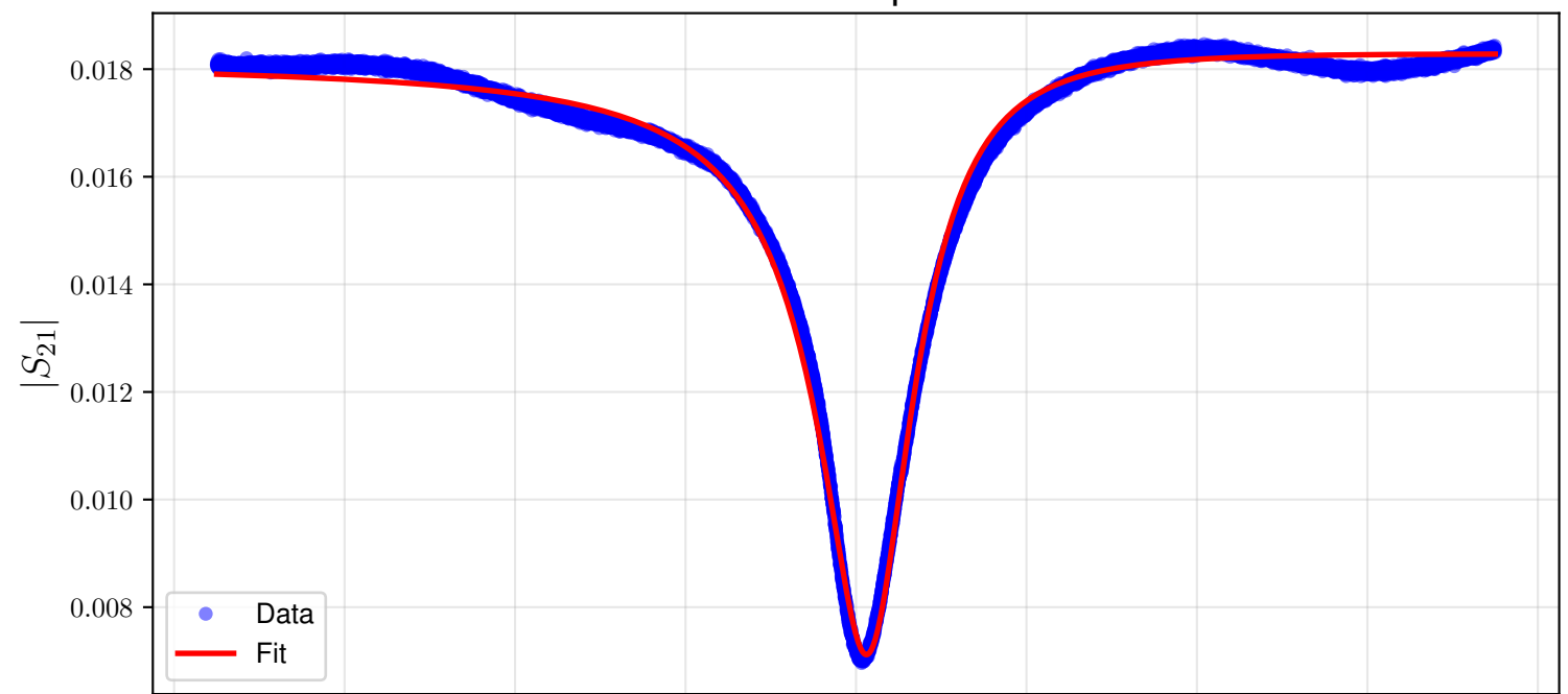
Resonance Fit - Temperature: 975mK
