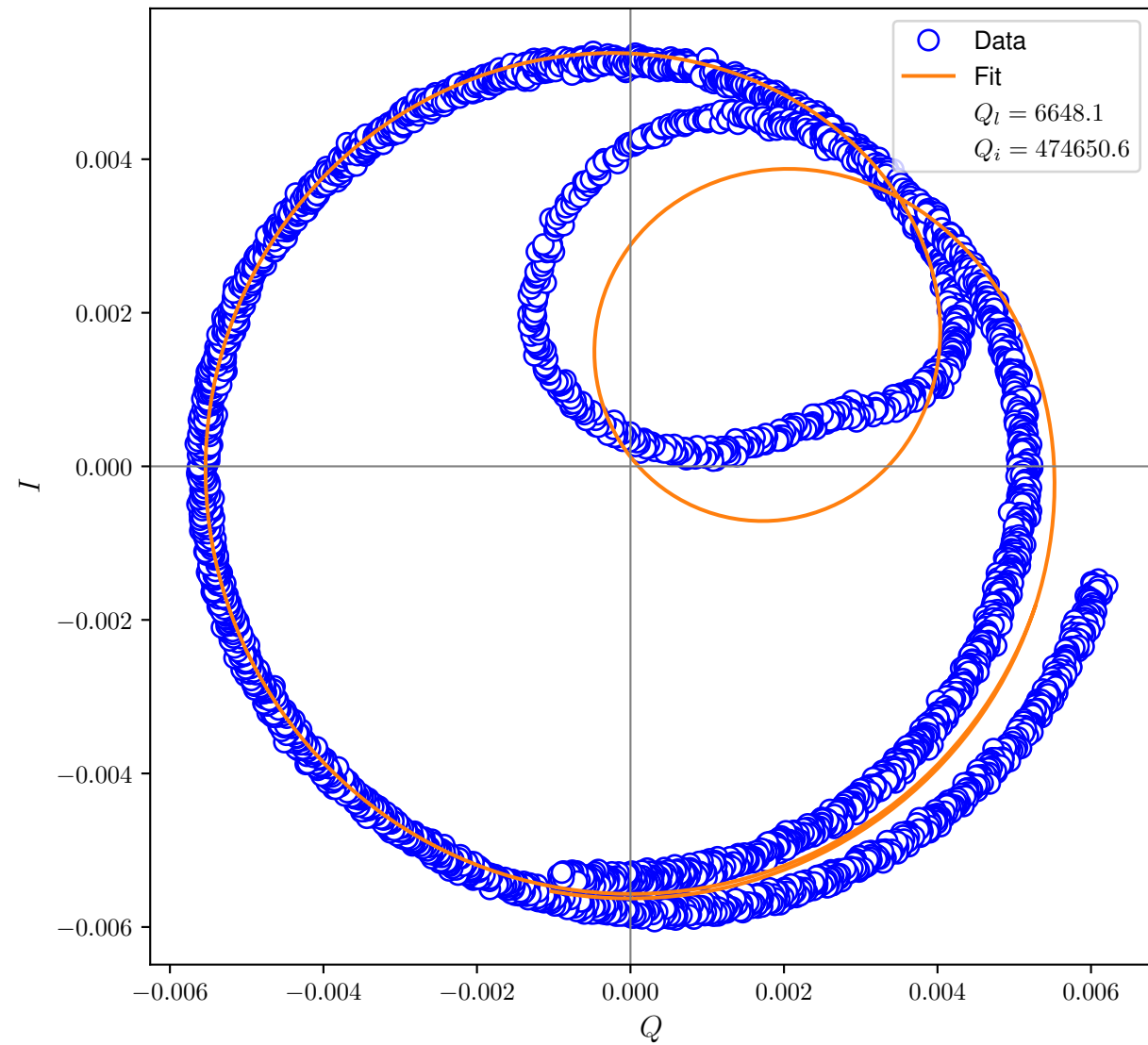
I-Q Plot
