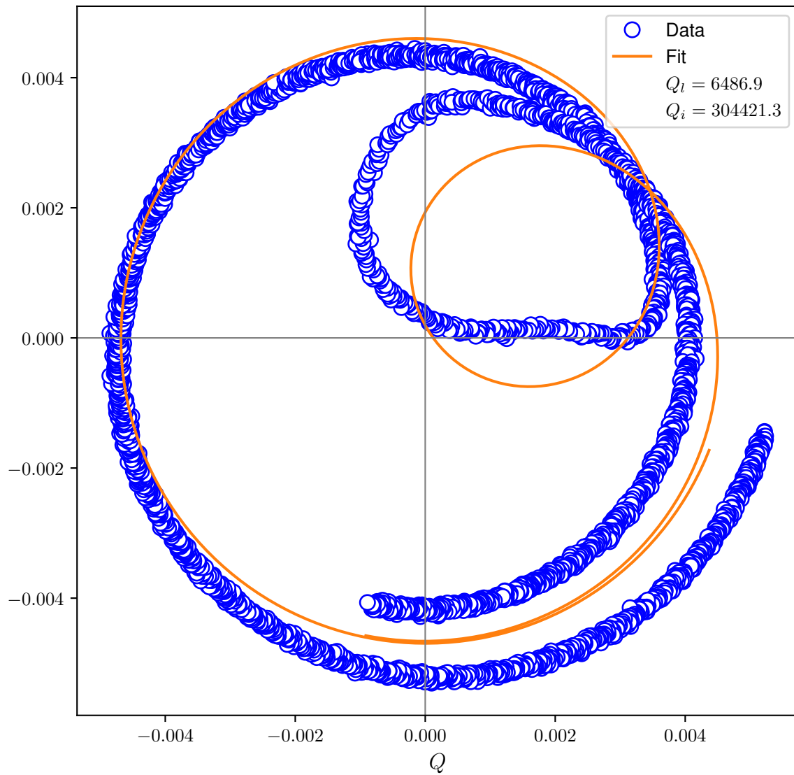
I-Q Plot
