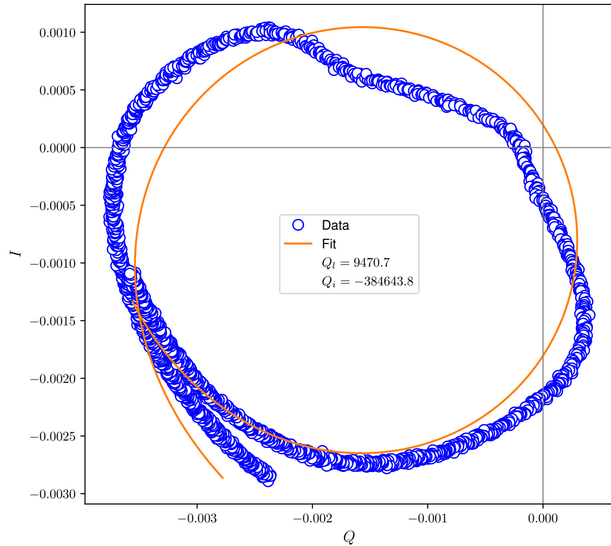
I-Q Plot
