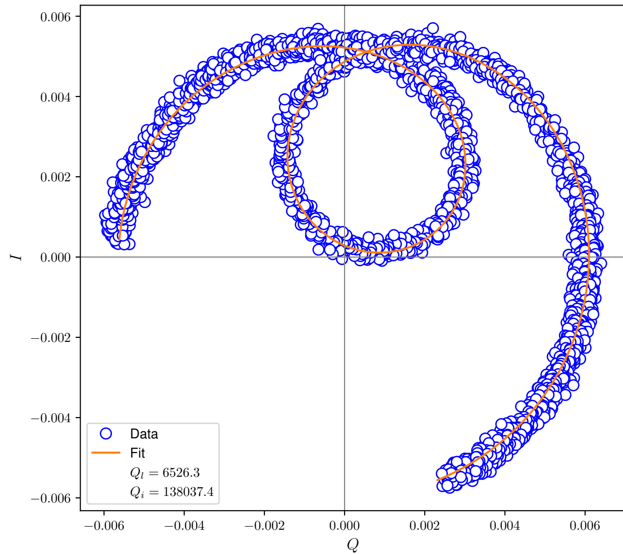
I-Q Plot
