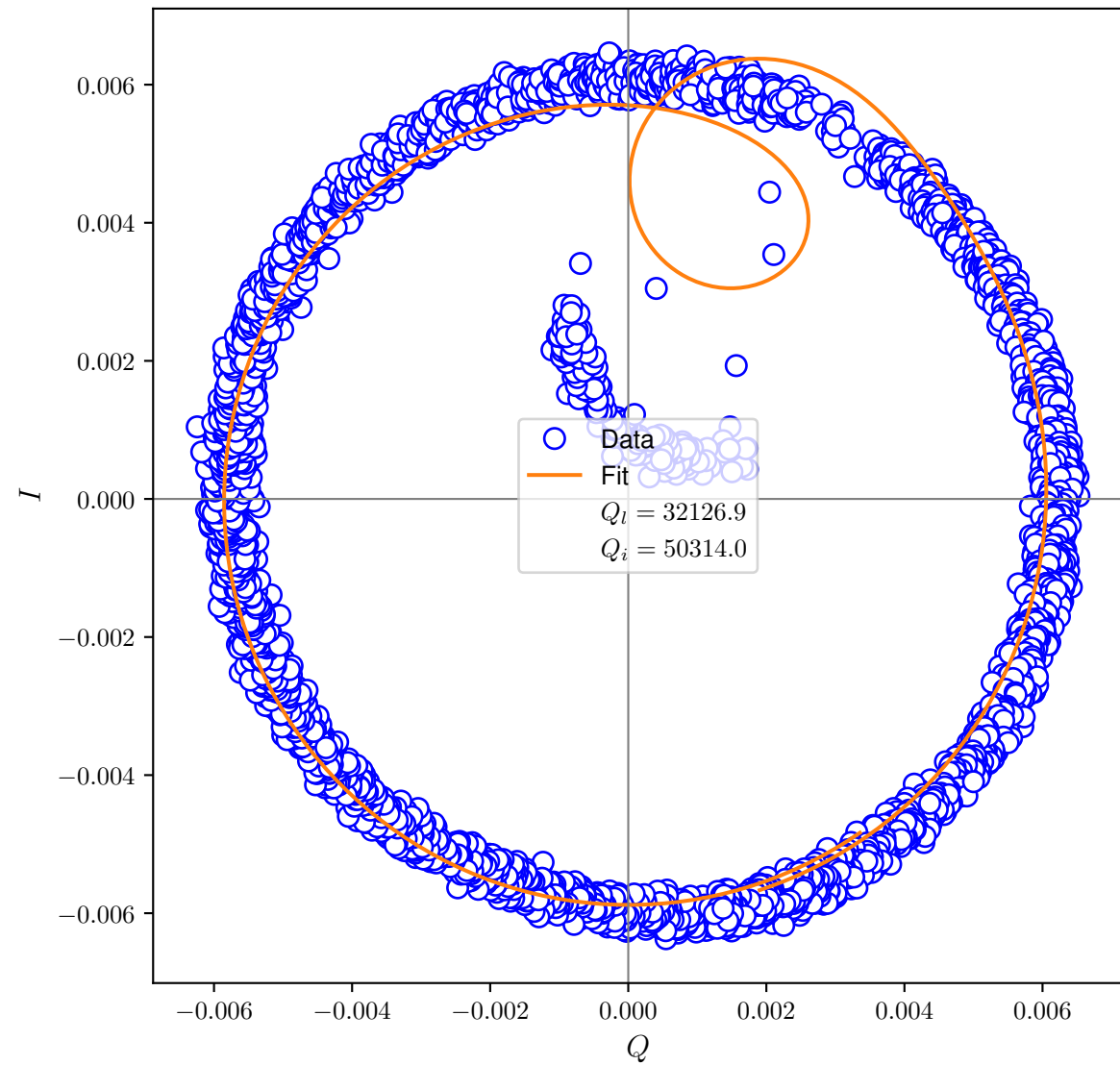
I-Q Plot
