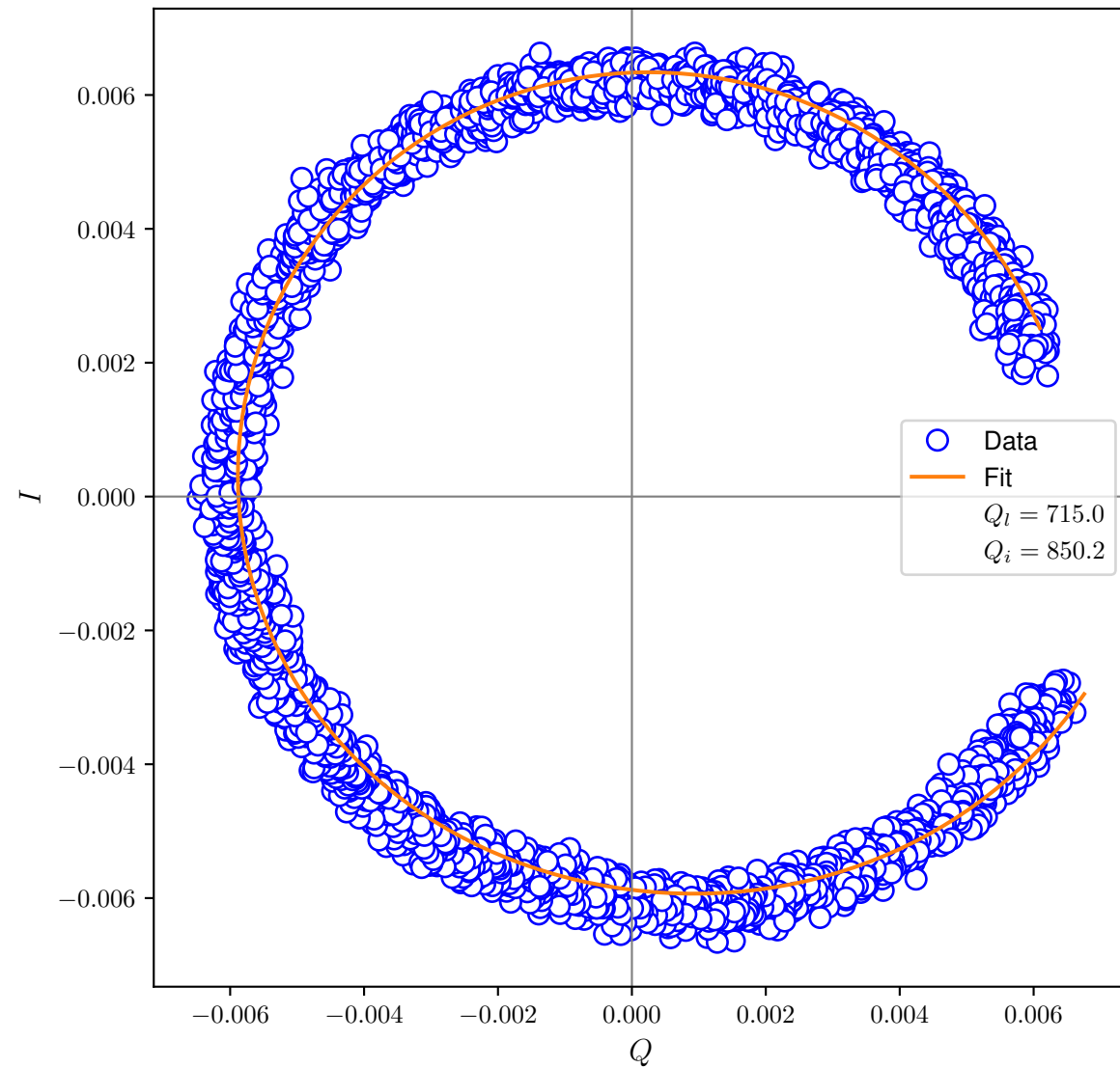
I-Q Plot
