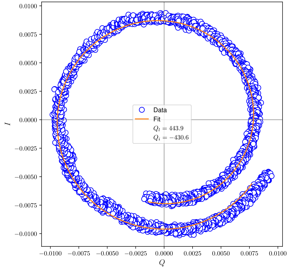
I-Q Plot
