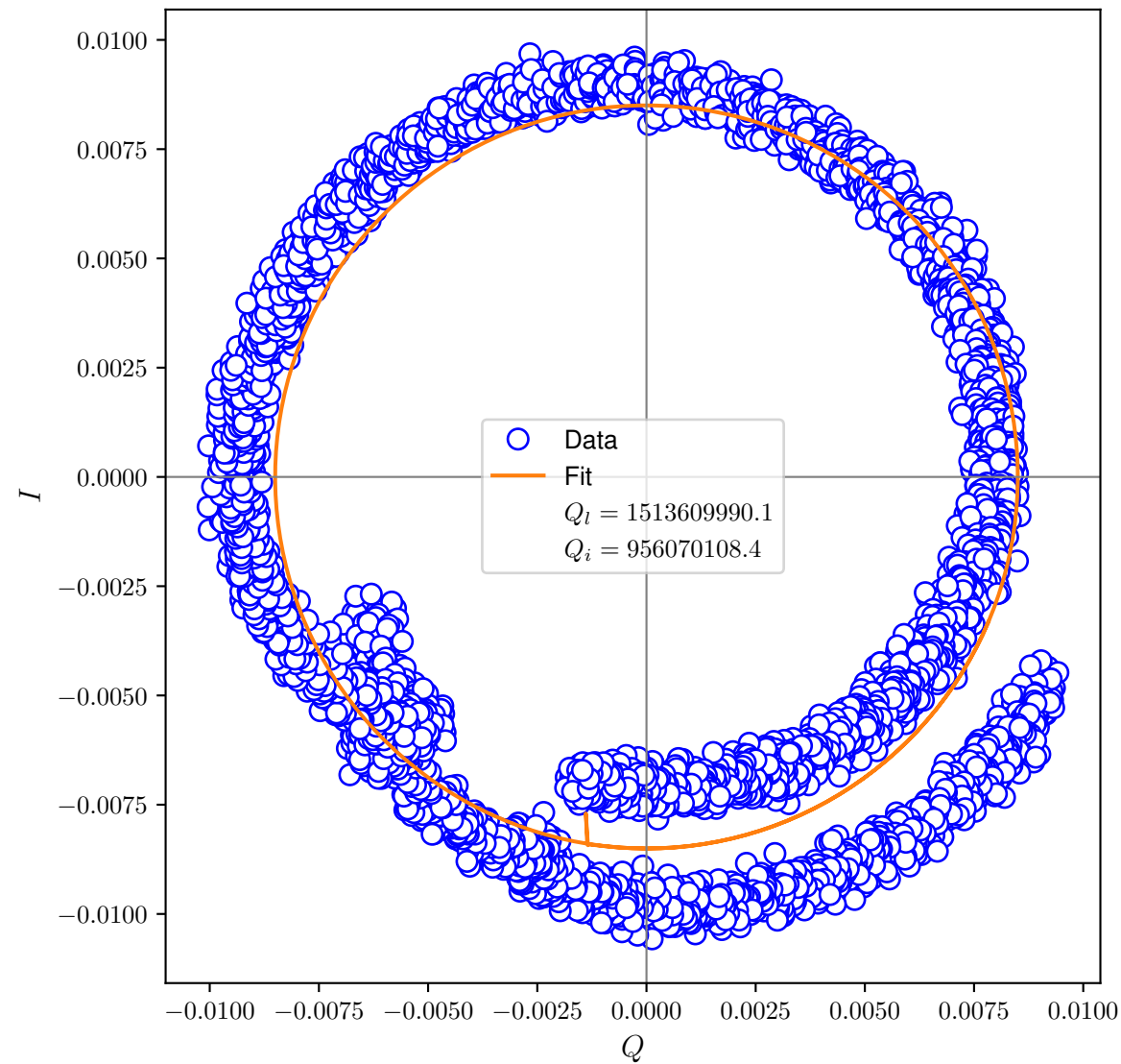
I-Q Plot
