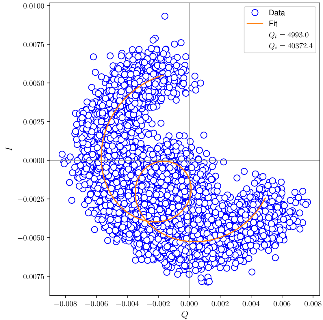
I-Q Plot
