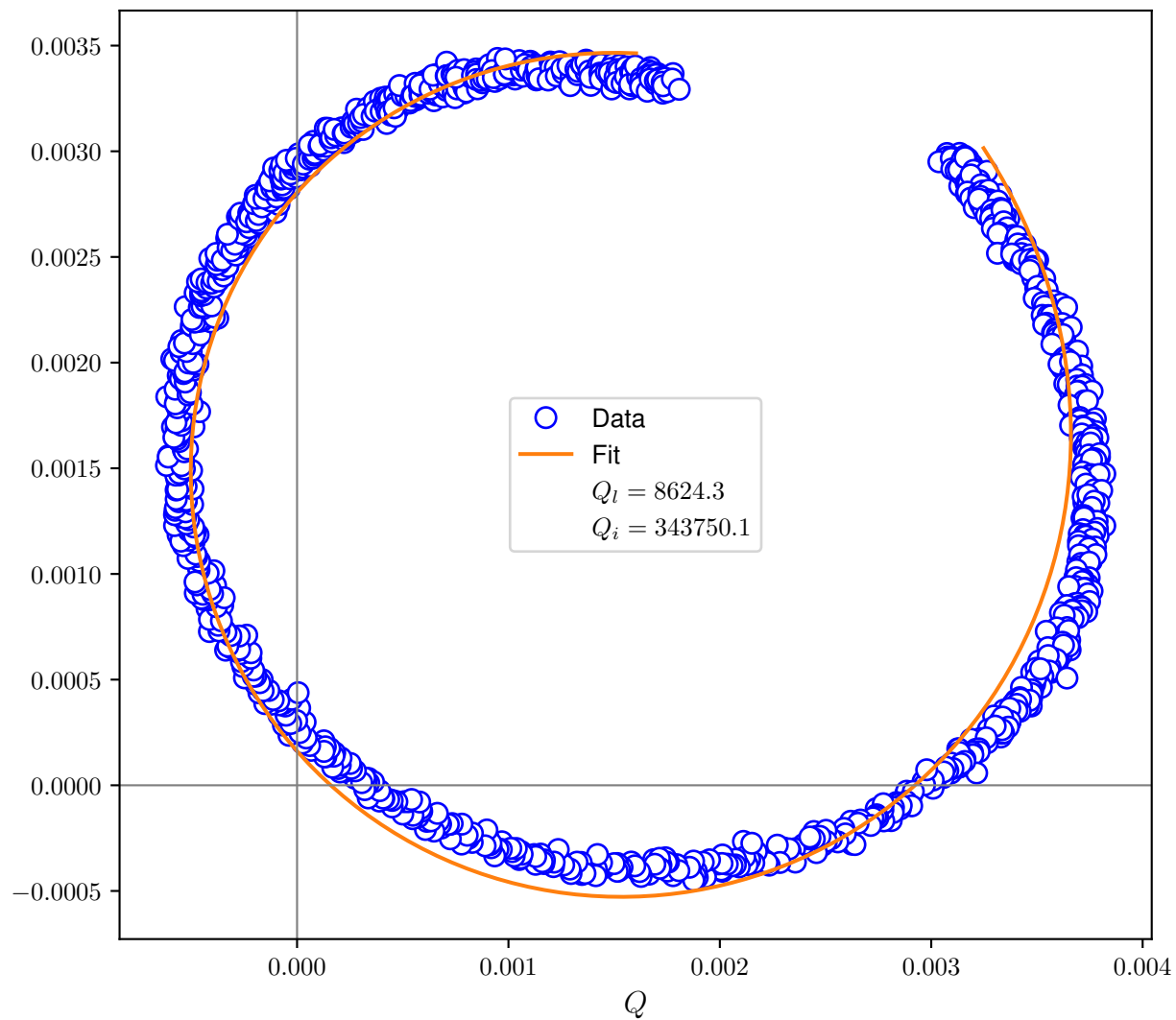
I-Q Plot
